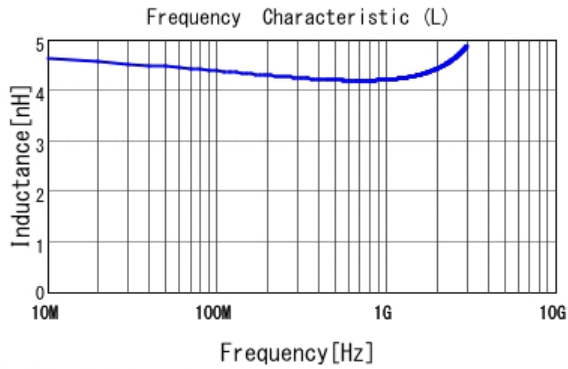
■ LQP03TN4N2B02 L
