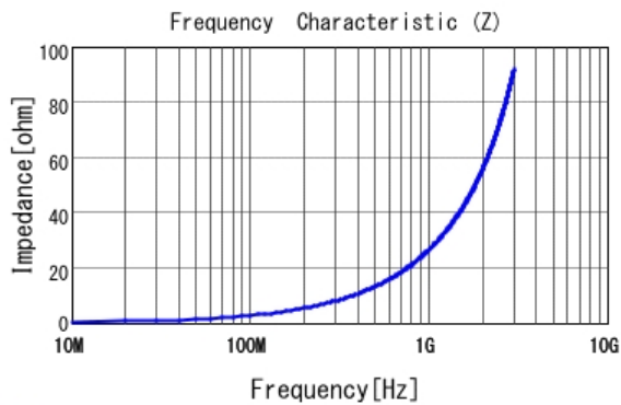
■ LQP03TN4N2B02 |Z|
