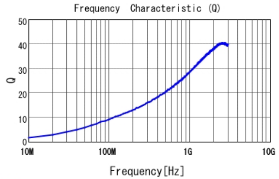
■ LQP03TN4N2B02 Q
