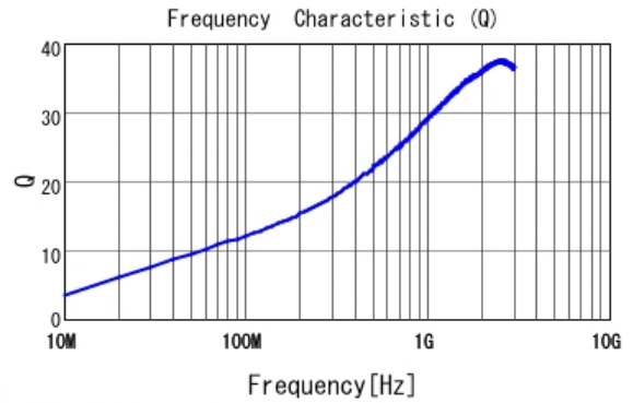
■ LQP03TN5N1J02 Q
