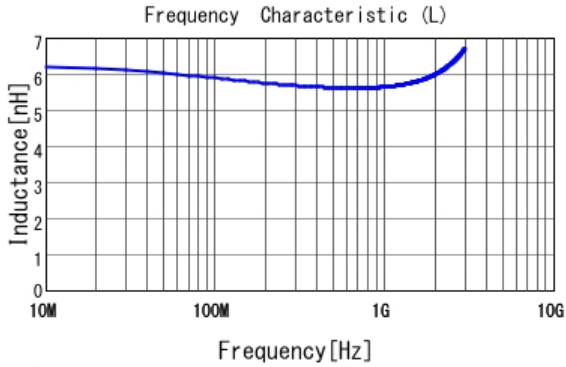
■ LQP03TN5N6H02 L
