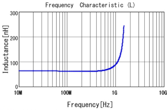
■ LQP03TN62NH02 L
