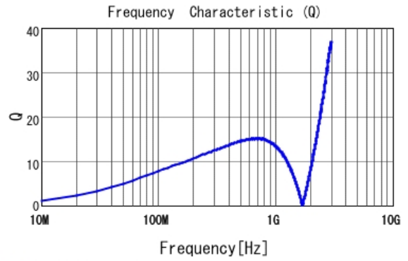
■ LQP03TN62NH02 Q
