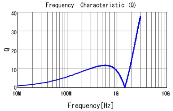
■ LQP03TN68NJ02 Q
