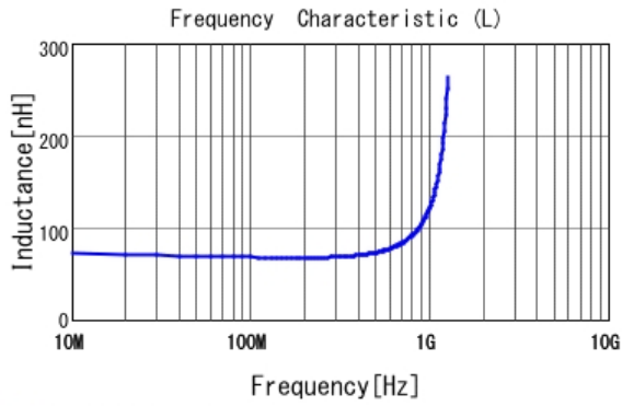
■ LQP03TN68NJ02 L
