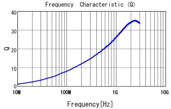
■ LQP03TN6N2J02 Q
