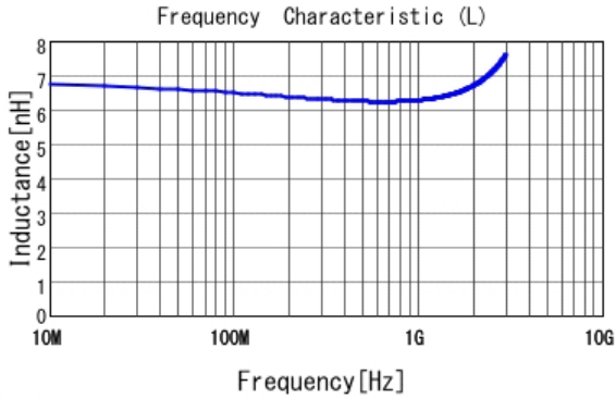
■ LQP03TN6N2J02 L
