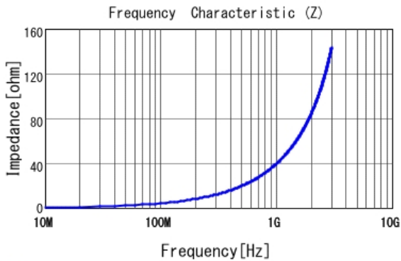
■ LQP03TN6N2J02 |Z|
