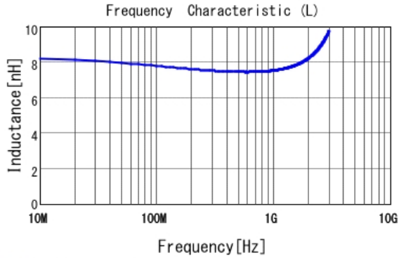
■ LQP03TN7N5H02 L
