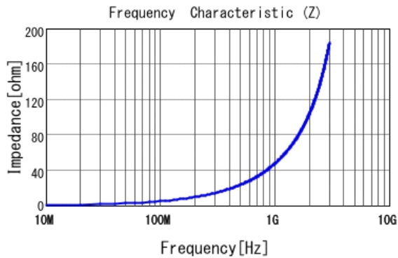
■ LQP03TN7N5H02 |Z|
