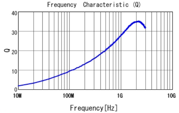
■ LQP03TN7N5H02 Q
