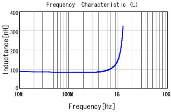
■ LQP03TN82NH02 L
