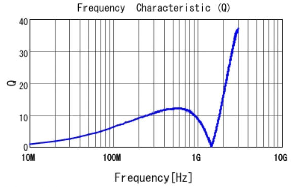
■ LQP03TN82NH02 Q
