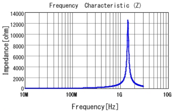
■ LQP03TN82NH02 |Z|
