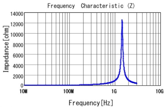
■ LQP03TN82NJ02 |Z|
