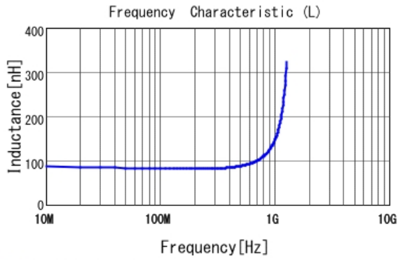
■ LQP03TN82NJ02 L
