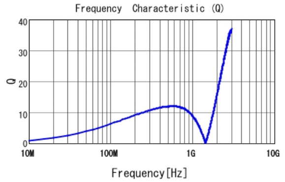
■ LQP03TN82NJ02 Q
