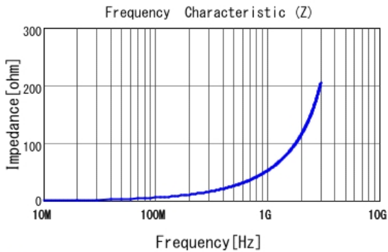
■ LQP03TN8N2J02 |Z|
