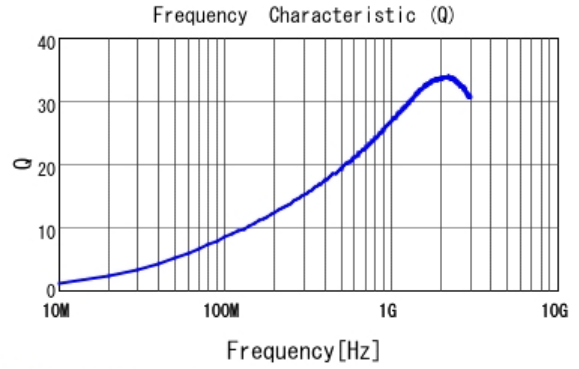
■ LQP03TN8N2J02 Q
