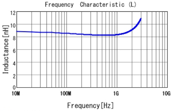
■ LQP03TN8N2J02 L
