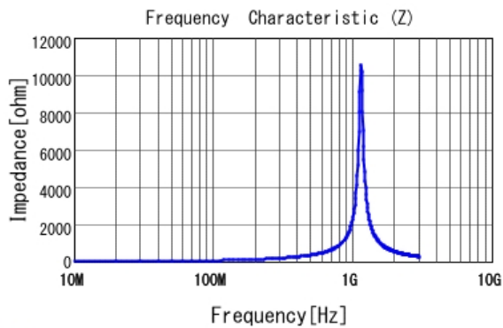
■ LQP03TNR10J02 |Z|
