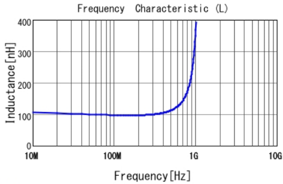
■ LQP03TNR10J02 L
