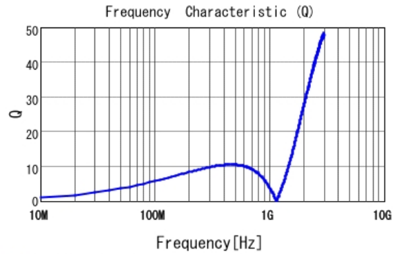
■ LQP03TNR10J02 Q
