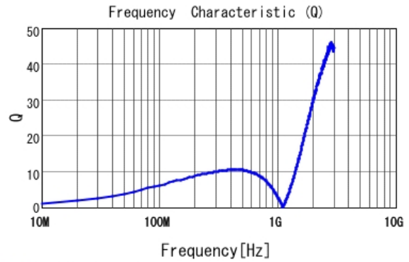
■ LQP03TNR11J02 Q
