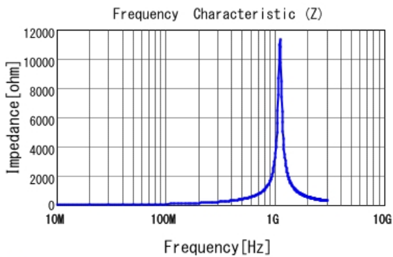
■ LQP03TNR11J02 |Z|
