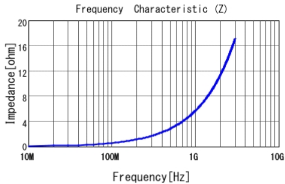
■ LQP03TQ0N9W02 |Z|
