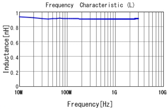
■ LQP03TQ0N9W02 L
