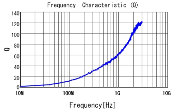
■ LQP03TQ0N9W02 Q
