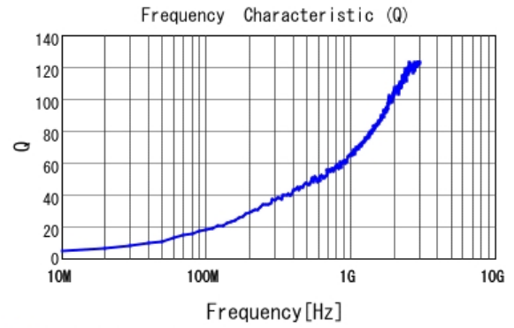
■ LQP03TQ1N0B02 Q
