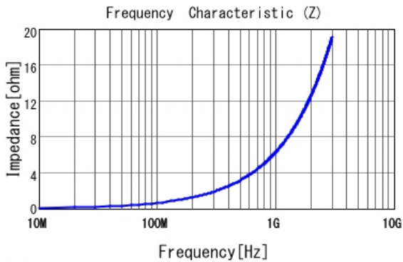
■ LQP03TQ1N0B02 |Z|
