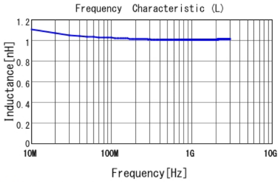
■ LQP03TQ1N0B02 L
