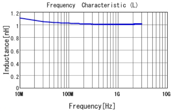
■ LQP03TQ1N0W02 L
