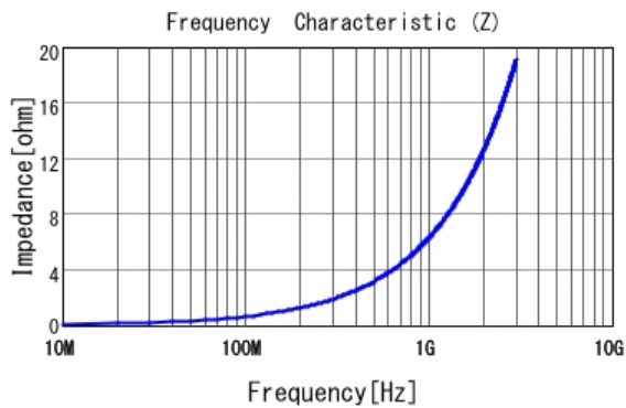
■ LQP03TQ1N0W02 |Z|
