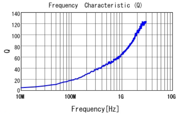
■ LQP03TQ1N0W02 Q
