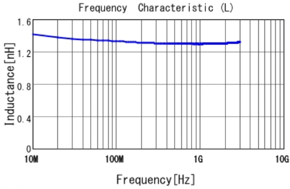
■ LQP03TQ1N3B02 L
