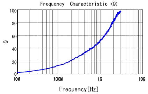
■ LQP03TQ1N3B02 Q
