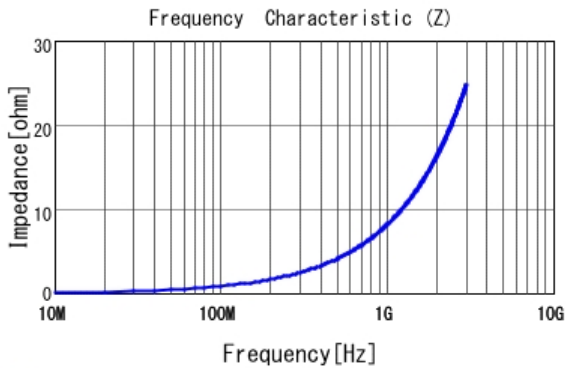
■ LQP03TQ1N3B02 |Z|
