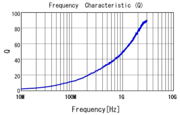
■ LQP03TQ1N4W02 Q
