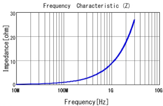
■ LQP03TQ1N4W02 |Z|
