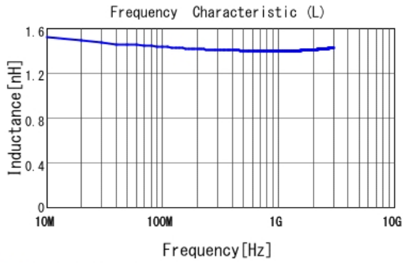
■ LQP03TQ1N4W02 L
