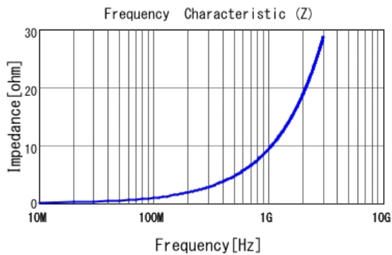
■ LQP03TQ1N5W02 |Z|
