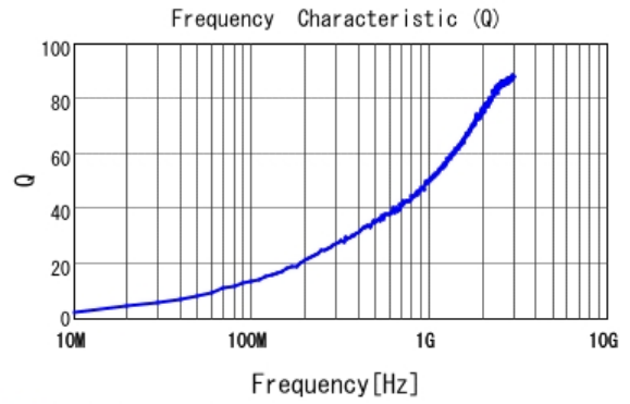
■ LQP03TQ1N5W02 Q
