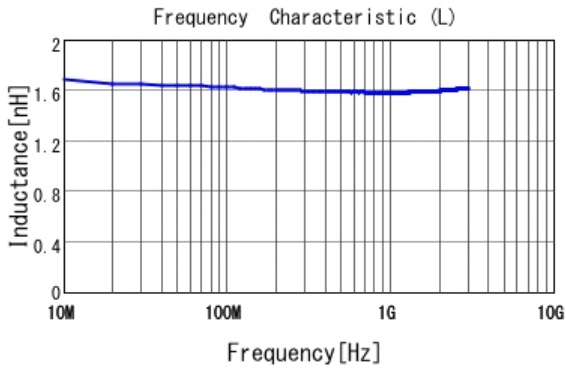
■ LQP03TQ1N6C02 L
