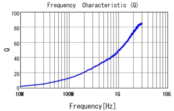
■ LQP03TQ1N6C02 Q
