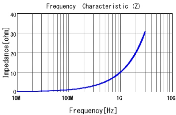
■ LQP03TQ1N6C02 |Z|
