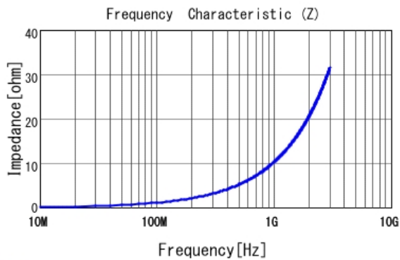
■ LQP03TQ1N7B02 |Z|
