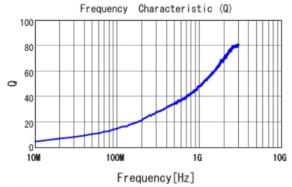
■ LQP03TQ1N7B02 Q
