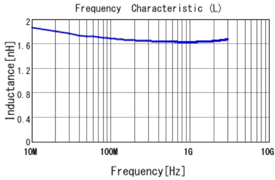
■ LQP03TQ1N7B02 L
