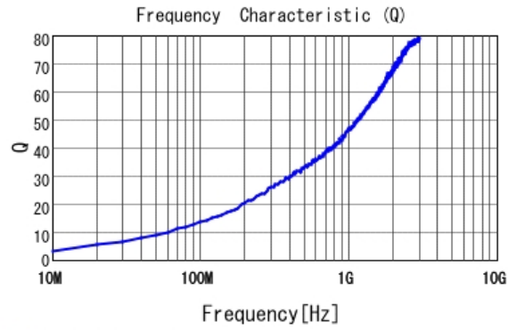
■ LQP03TQ1N8B02 Q
