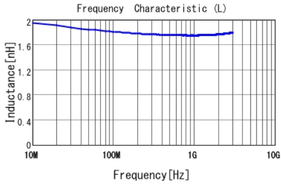
■ LQP03TQ1N8B02 L
