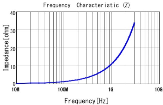
■ LQP03TQ1N8B02 |Z|
