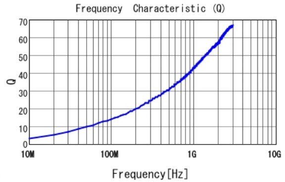
■ LQP03TQ2N5B02 Q
