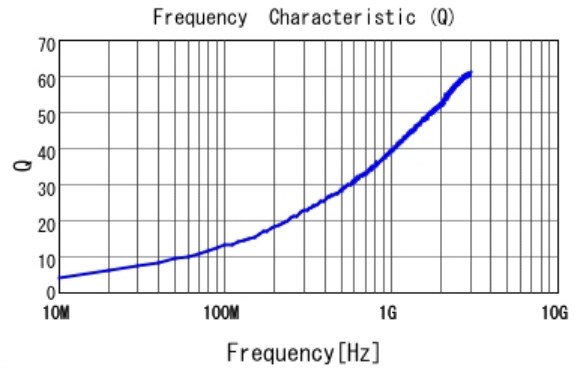
■ LQP03TQ2N7B02 Q
