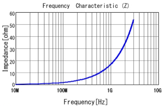
■ LQP03TQ2N7B02 |Z|
