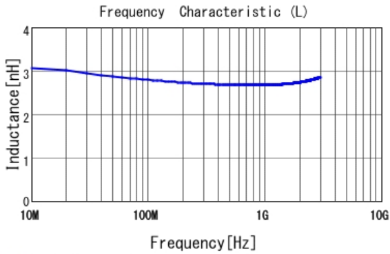
■ LQP03TQ2N7B02 L
