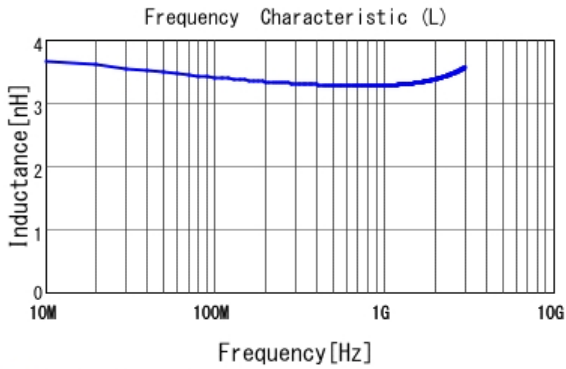
■ LQP03TQ3N3B02 L
