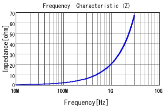
■ LQP03TQ3N3B02 |Z|
