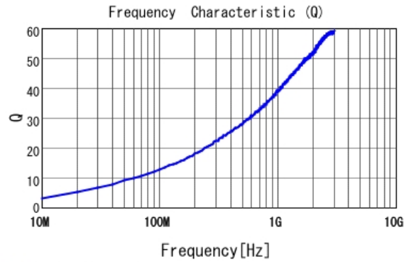
■ LQP03TQ3N3B02 Q
