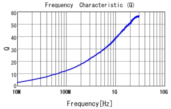
■ LQP03TQ3N6B02 Q
