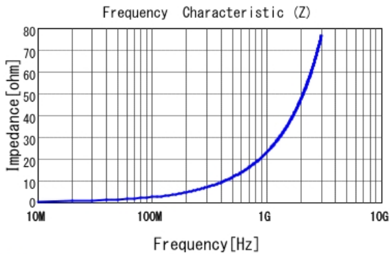
■ LQP03TQ3N6B02 |Z|
