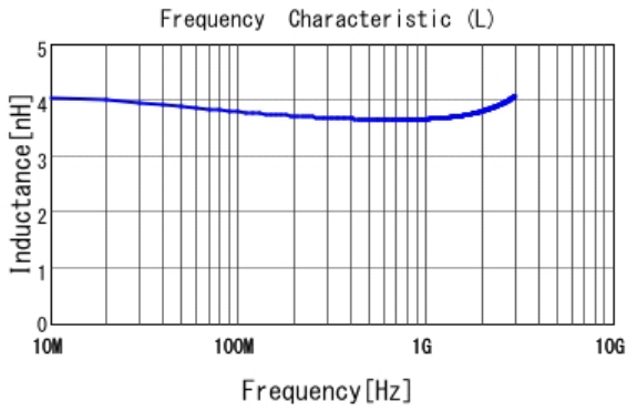
■ LQP03TQ3N6B02 L
