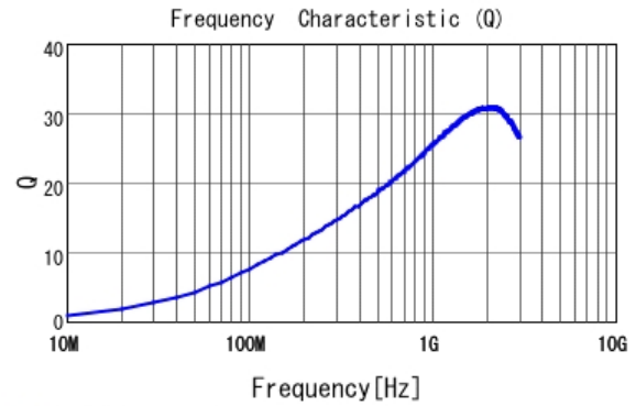
■ LQP15MN10NG02 Q
