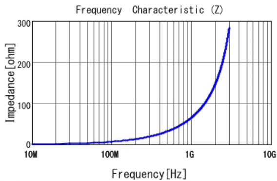
■ LQP15MN10NG02 |Z|
