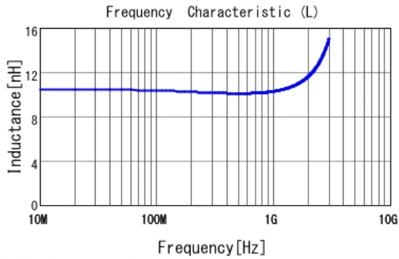
■ LQP15MN10NG02 L
