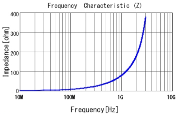
■ LQP15MN12NG02 |Z|
