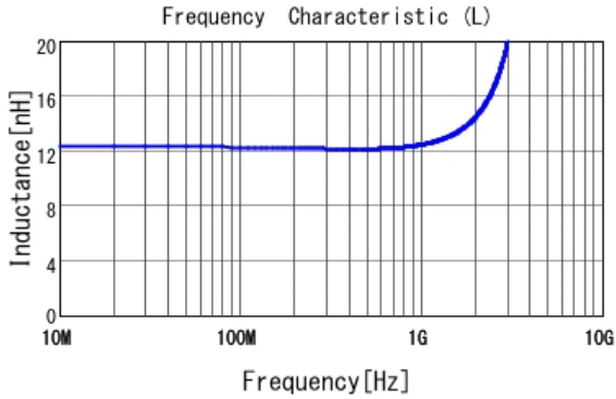
■ LQP15MN12NG02 L
