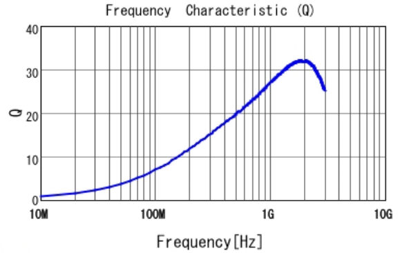
■ LQP15MN12NG02 Q
