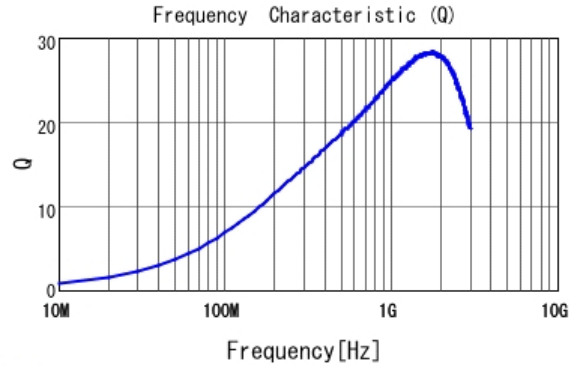
■ LQP15MN15NG02 Q
