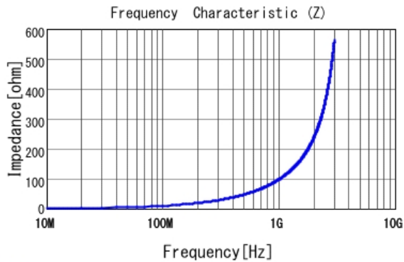
■ LQP15MN15NG02 |Z|
