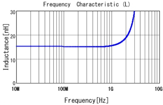
■ LQP15MN15NG02 L
