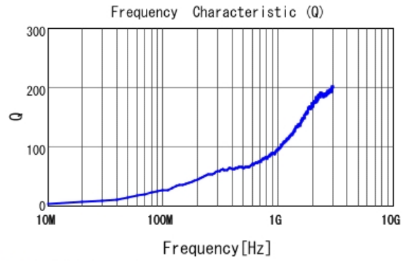
■ LQP15MN1N0B02 Q
