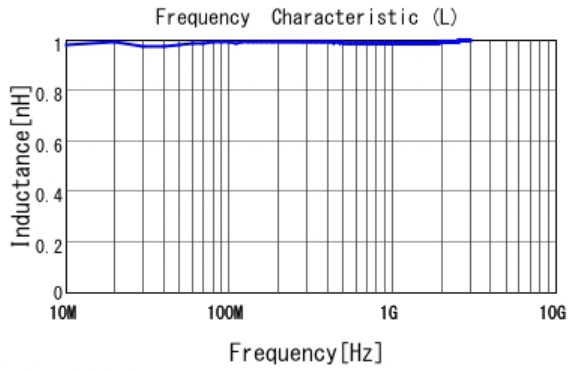
■ LQP15MN1N0B02 L
