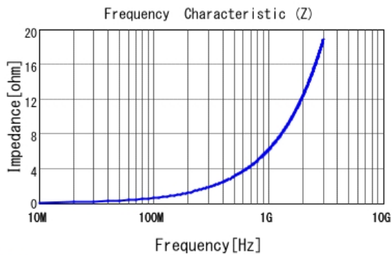
■ LQP15MN1N0B02 |Z|
