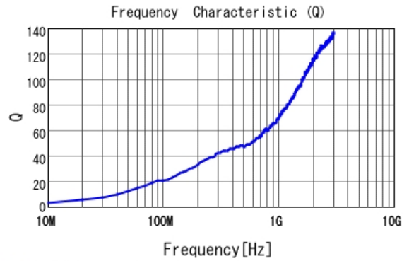
■ LQP15MN1N1B02 Q
