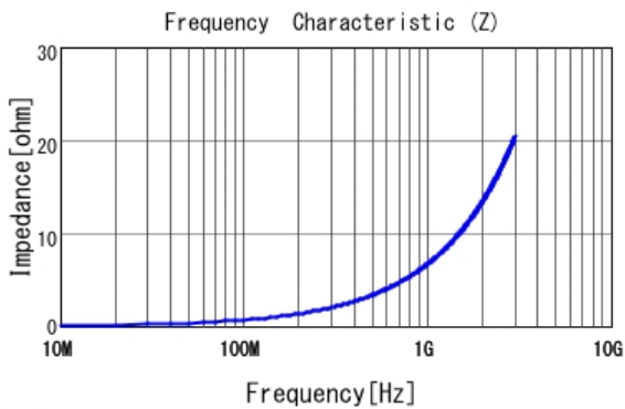
■ LQP15MN1N1B02 |Z|
