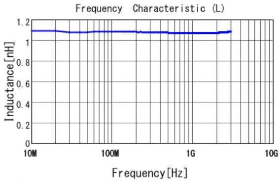
■ LQP15MN1N1B02 L
