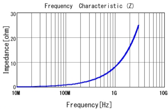
■ LQP15MN1N3B02 |Z|
