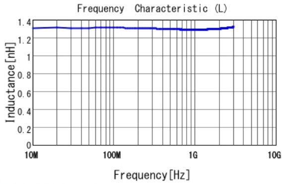
■ LQP15MN1N3B02 L
