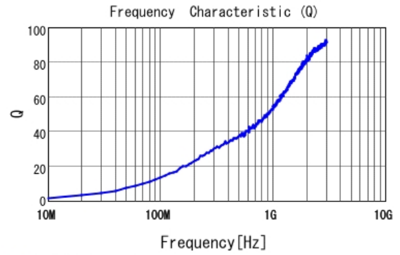
■ LQP15MN1N3B02 Q
