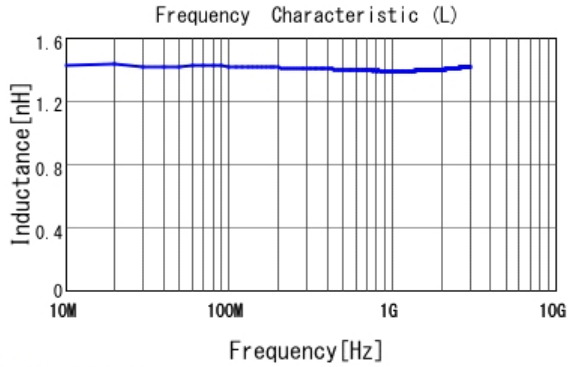
■ LQP15MN1N4W02 L
