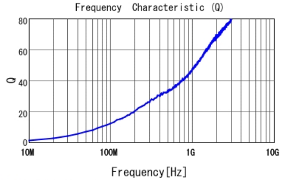
■ LQP15MN1N4W02 Q
