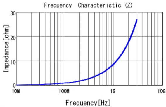
■ LQP15MN1N4W02 |Z|
