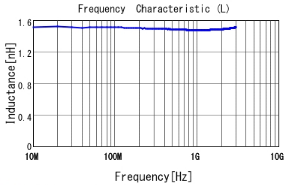
■ LQP15MN1N5B02 L
