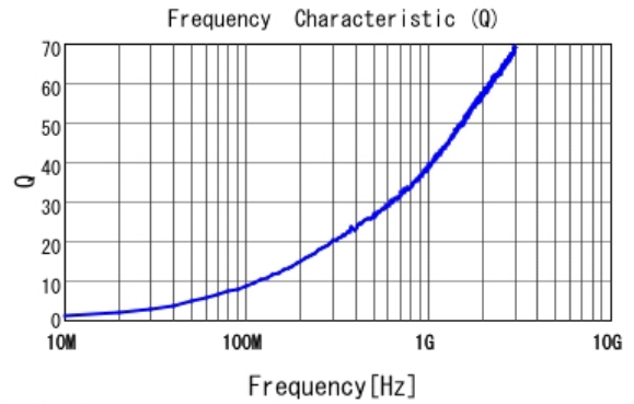
■ LQP15MN1N5B02 Q
