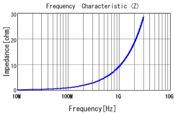
■ LQP15MN1N5W02 |Z|
