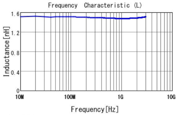
■ LQP15MN1N5W02 L
