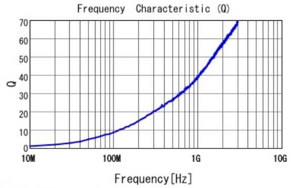
■ LQP15MN1N5W02 Q
