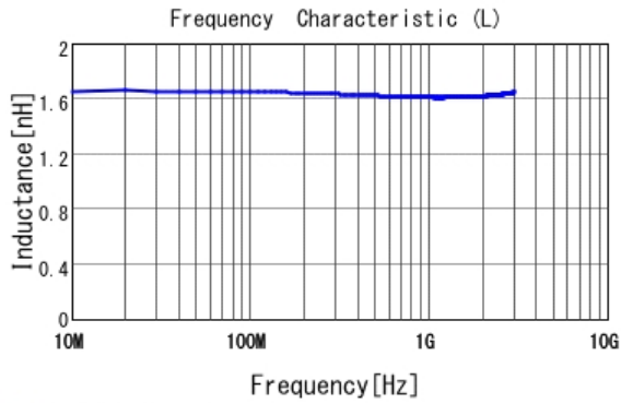
■ LQP15MN1N6B02 L
