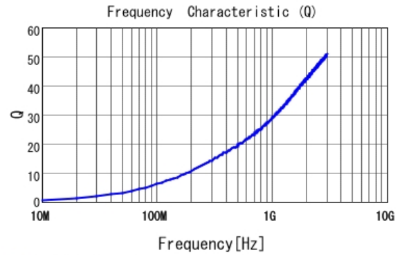
■ LQP15MN1N6B02 Q
