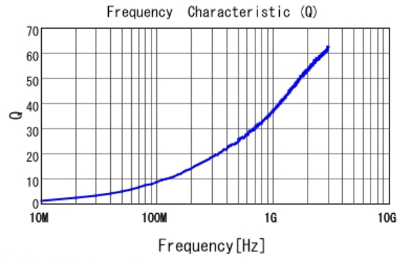
■ LQP15MN1N8B02 Q
