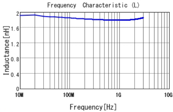
■ LQP15MN1N8B02 L
