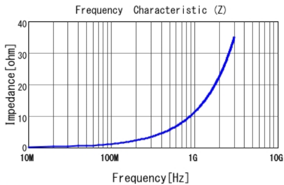
■ LQP15MN1N8B02 |Z|
