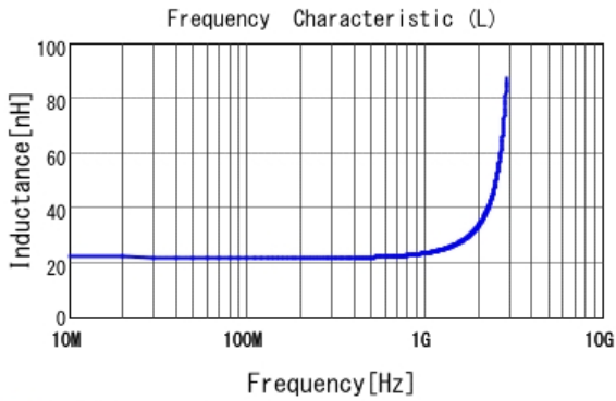
■ LQP15MN22NG02 L
