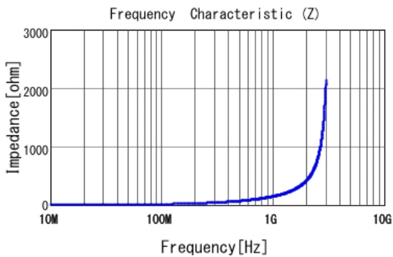
■ LQP15MN22NG02 |Z|
