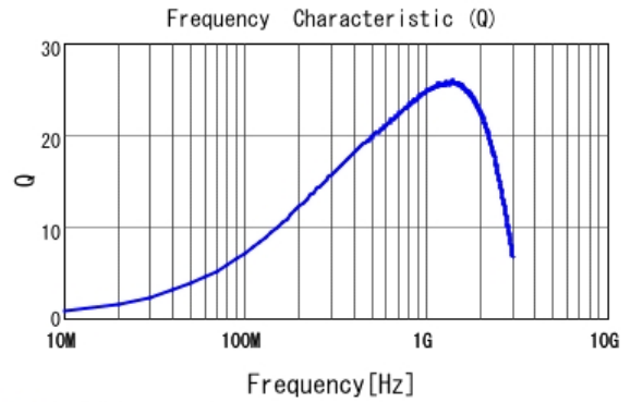
■ LQP15MN22NG02 Q
