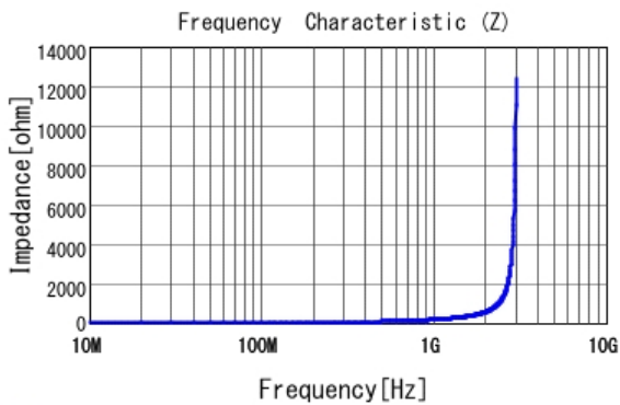
■ LQP15MN27NG02 |Z|
