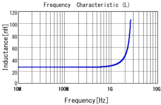
■ LQP15MN27NG02 L
