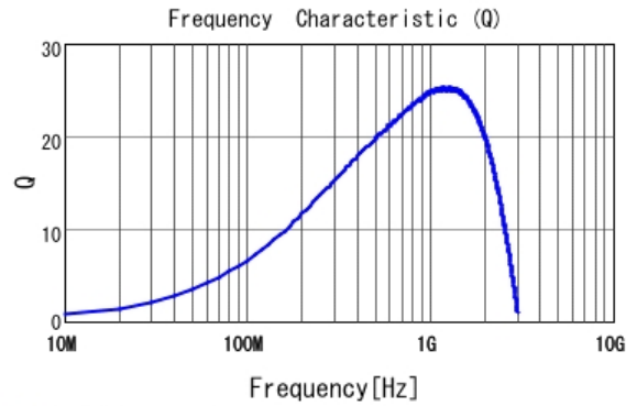
■ LQP15MN27NG02 Q
