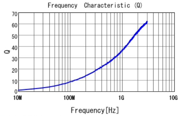
■ LQP15MN2N0B02 Q
