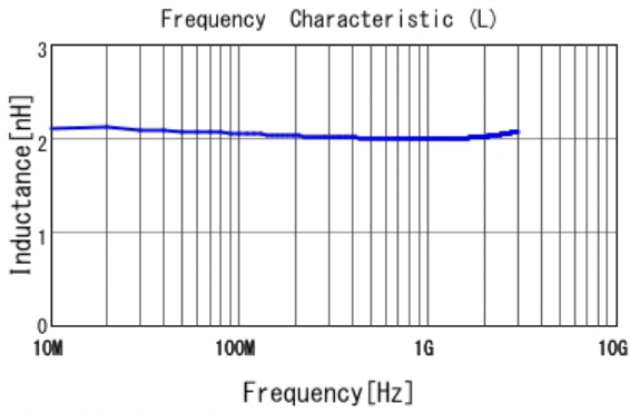
■ LQP15MN2N0B02 L
