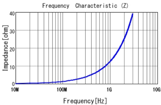
■ LQP15MN2N0W02 |Z|
