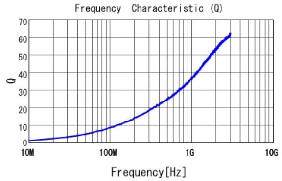
■ LQP15MN2N0W02 Q
