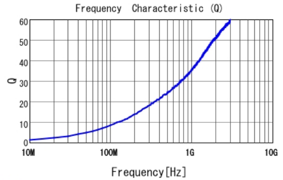
■ LQP15MN2N2B02 Q
