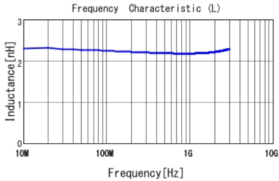
■ LQP15MN2N2B02 L
