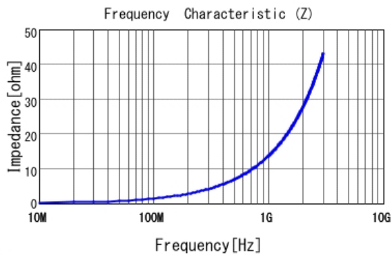
■ LQP15MN2N2B02 |Z|
