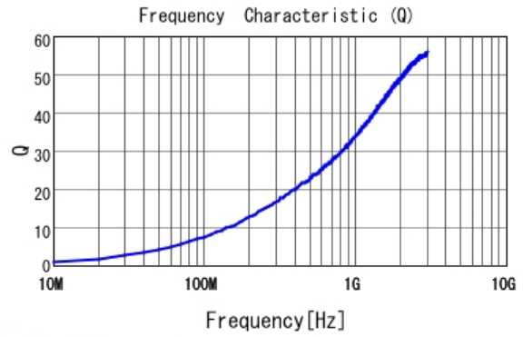
■ LQP15MN2N7W02 Q
