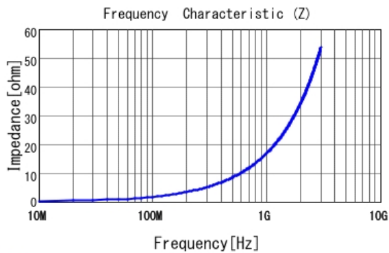
■ LQP15MN2N7W02 |Z|
