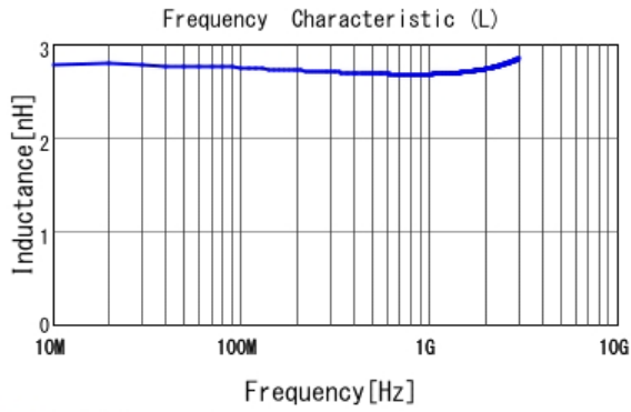
■ LQP15MN2N7W02 L
