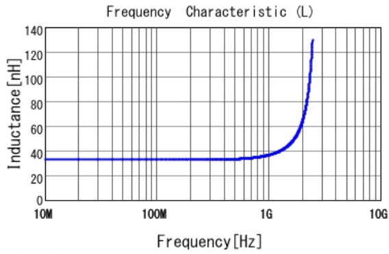
■ LQP15MN33NG02 L
