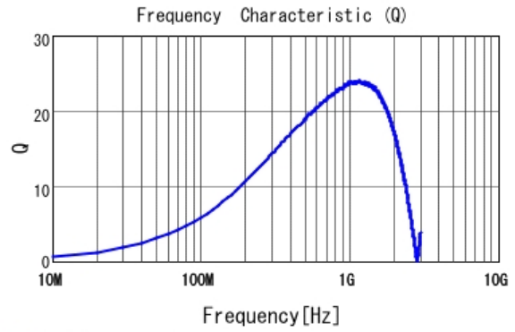
■ LQP15MN33NG02 Q
