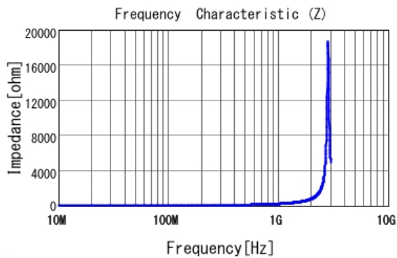
■ LQP15MN33NG02 |Z|
