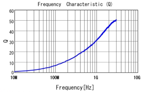
■ LQP15MN3N0B02 Q
