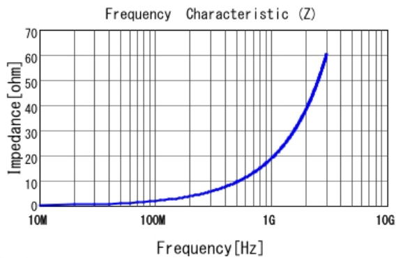
■ LQP15MN3N0B02 |Z|
