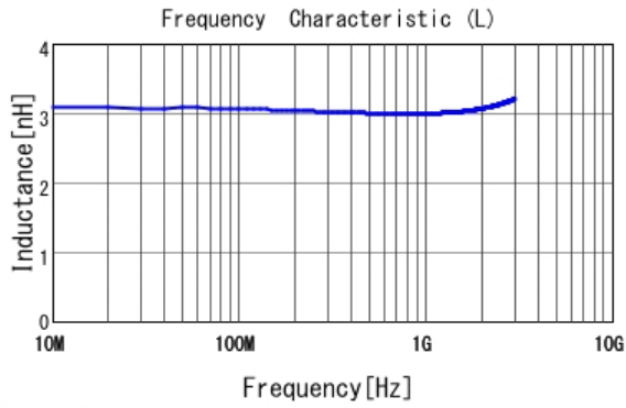
■ LQP15MN3N0B02 L
