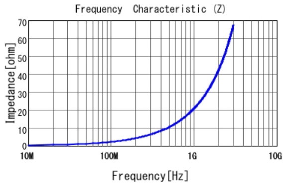
■ LQP15MN3N3B02 |Z|
