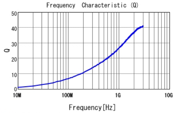
■ LQP15MN3N3B02 Q
