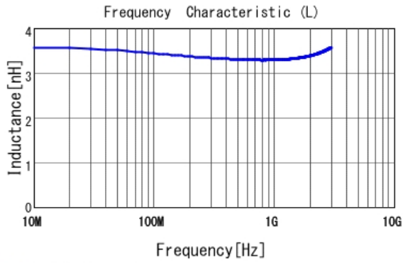
■ LQP15MN3N3B02 L
