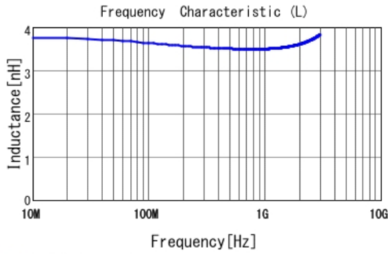
■ LQP15MN3N5W02 L
