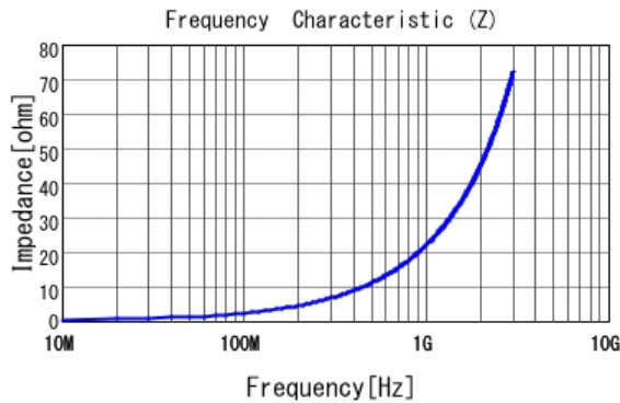
■ LQP15MN3N5W02 |Z|
