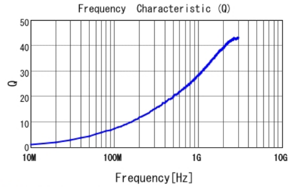
■ LQP15MN3N5W02 Q
