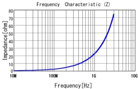
■ LQP15MN3N6B02 |Z|
