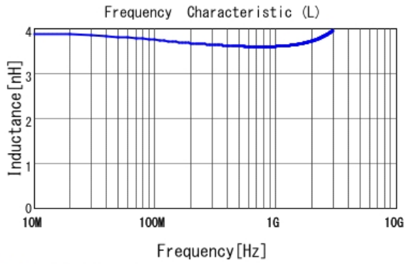
■ LQP15MN3N6B02 L
