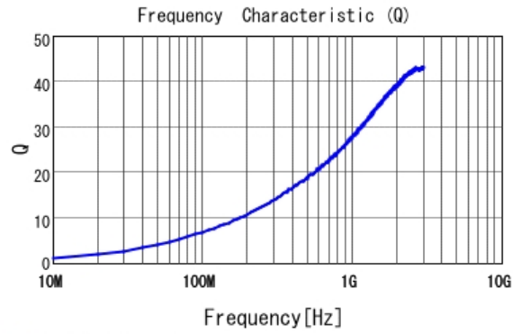
■ LQP15MN3N6B02 Q
