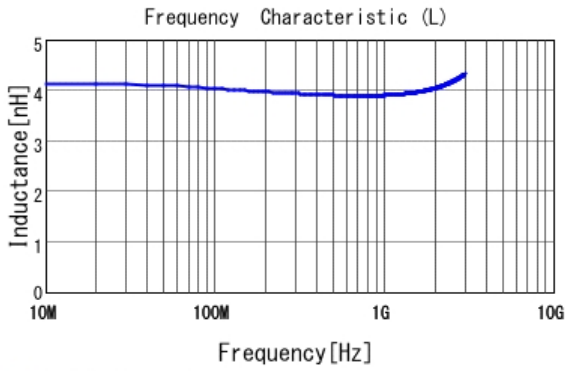
■ LQP15MN3N9B02 L
