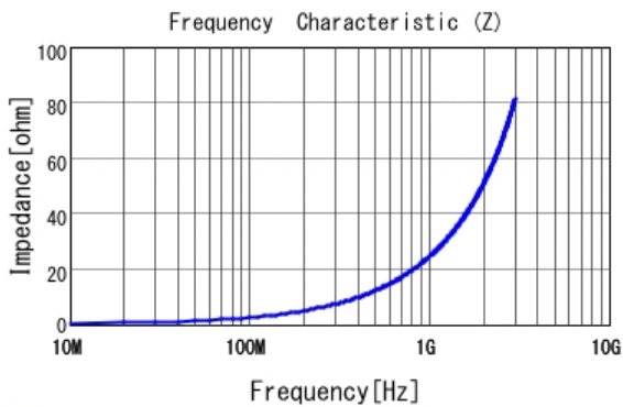
■ LQP15MN3N9B02 |Z|
