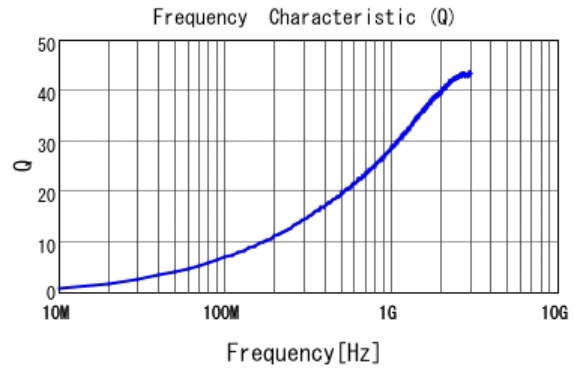
■ LQP15MN3N9B02 Q
