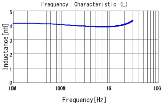
■ LQP15MN3N9W02 L
