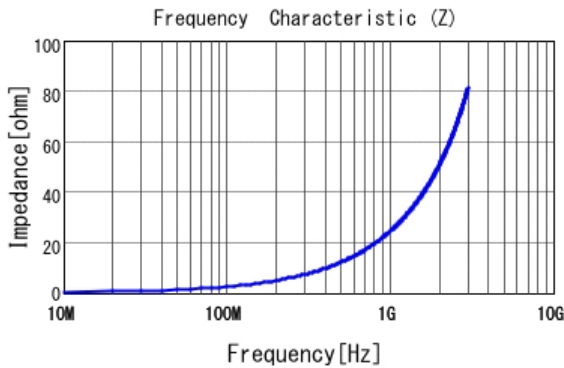
■ LQP15MN3N9W02 |Z|
