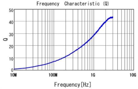
■ LQP15MN3N9W02 Q
