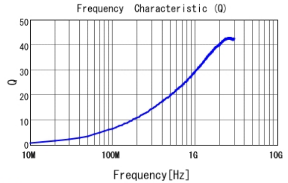
■ LQP15MN5N1B02 Q
