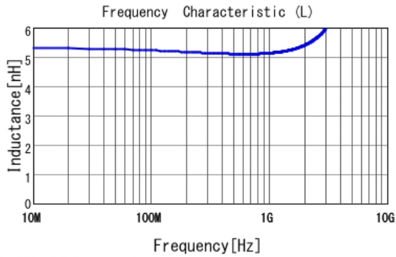
■ LQP15MN5N1B02 L
