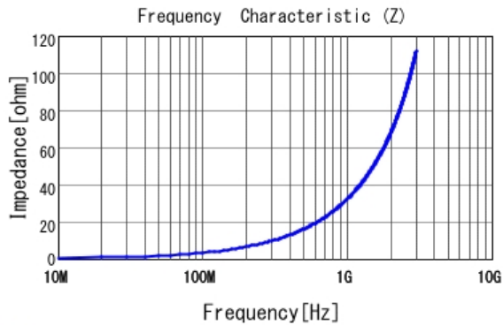
■ LQP15MN5N1B02 |Z|
